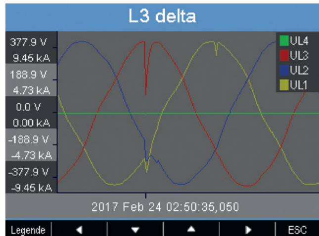
Fig.: Graphical representation of a transient
