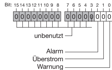
Abb. Alarm-Register
